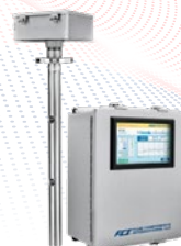
Multipoint thermal mass flow meter – FCI MT100
